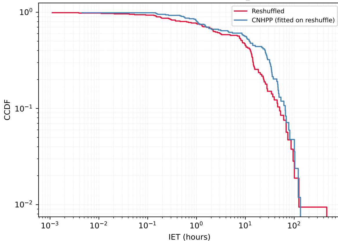
User 78947024 - Reshuffled vs CNHPP A_{\text{fit}}=0.1791
